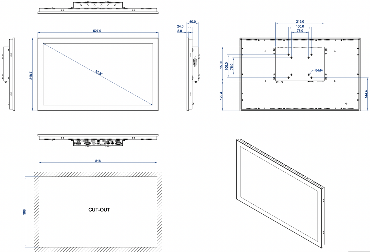
DIMENSIONAL DRAWING:TPC-DCS215R2
