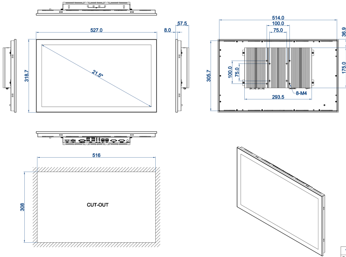
DIMENSIONAL DRAWING:TPC-DCS215
