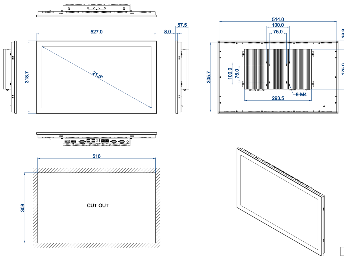
DIMENSIONAL DRAWING:TPC-DCS215
