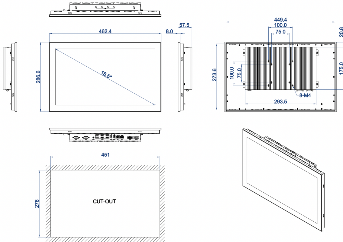
DIMENSIONAL DRAWING:TPC-DCS185E/T
