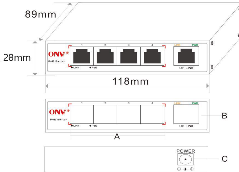
A. 4* PoE ports B. 60W PD power port C. DC power port
