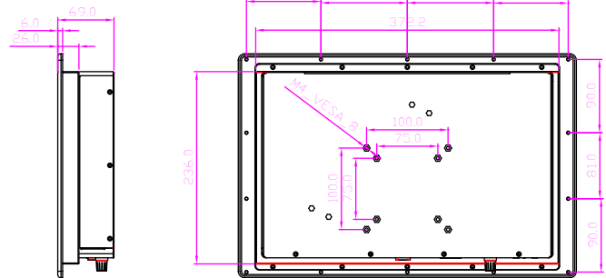
BACK VIEW
