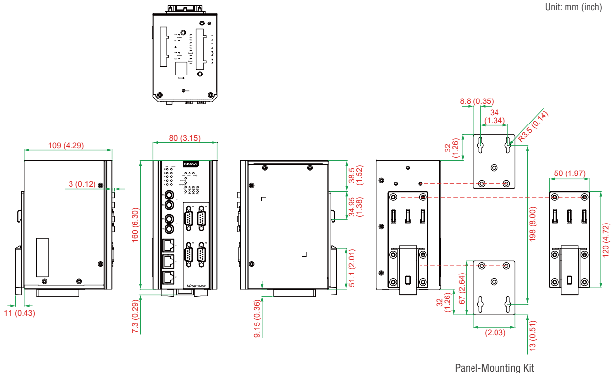
Panel-Mounting Kit
