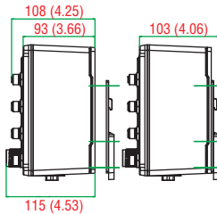
Side View (including DIN-Rail Mounting Kit)
