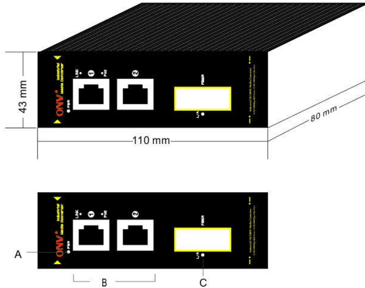
A. System Working Indicator B. 10/100M Rj45 PoE Port C. Uplink Optical SC Port
