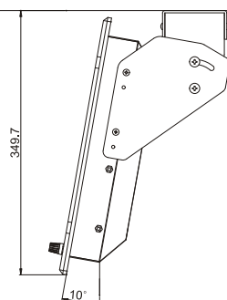
ROOF MOUNT
