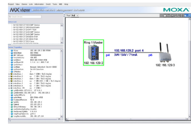
PoE Visualization
