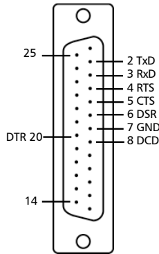
CBL-M37M25x4-30 (DB25 Male) (previously Opt4C) *30 cm Cable length *Reversible Connector Header
